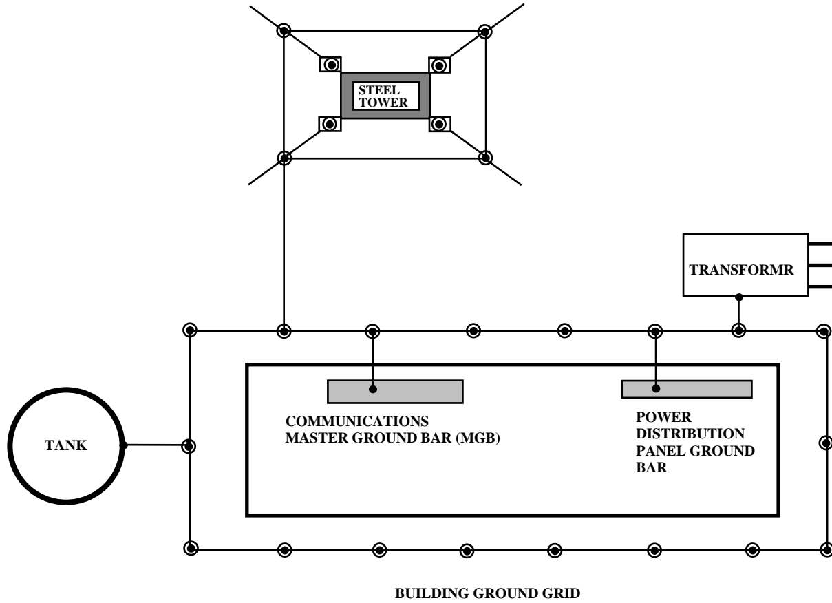
Figure 3 – AC/DC Grounding Arrangement
