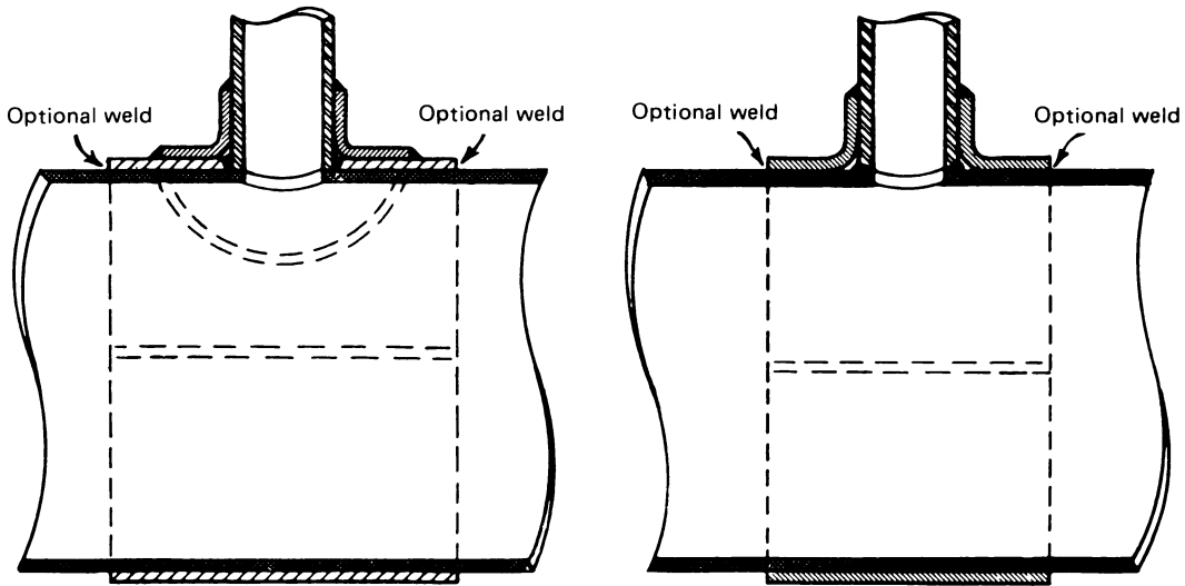
(c) Saddle and Sleeve Type [Note (3)]
