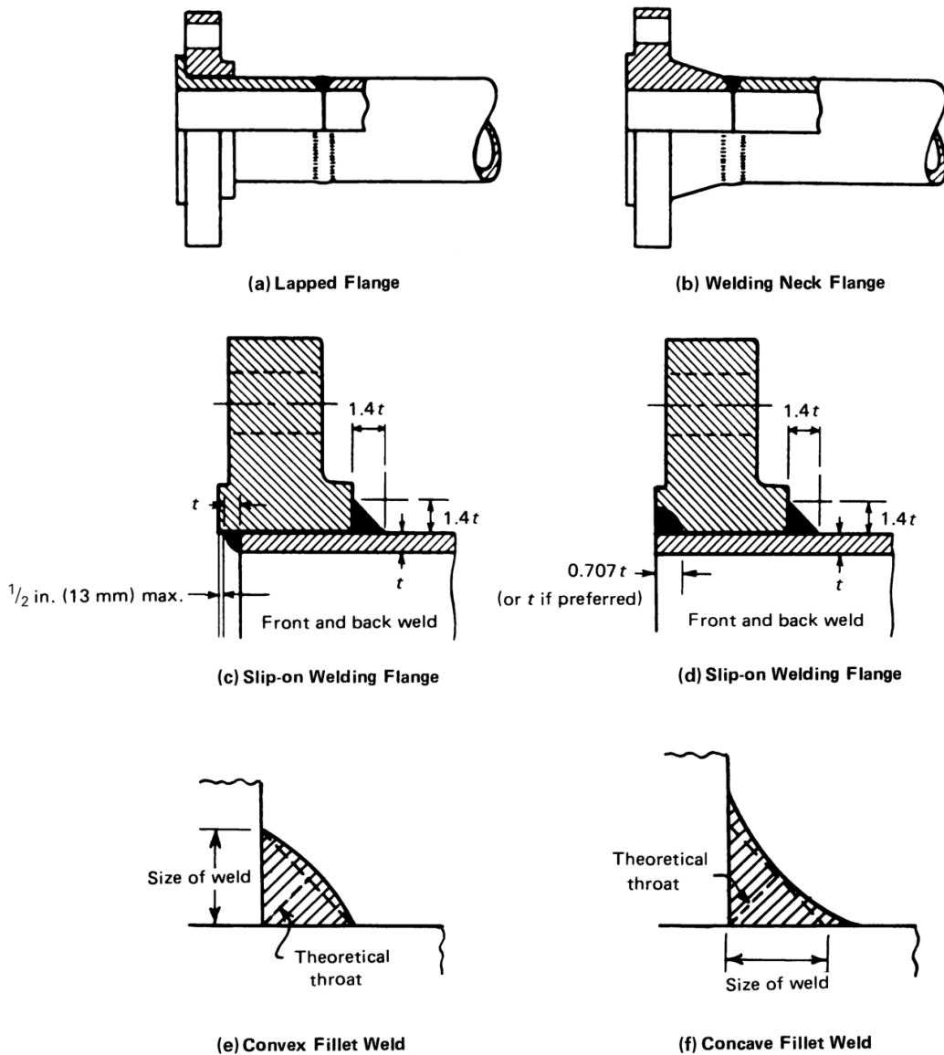
Figure 434.8.6-3 Recommended Attachment Details of Flanges
