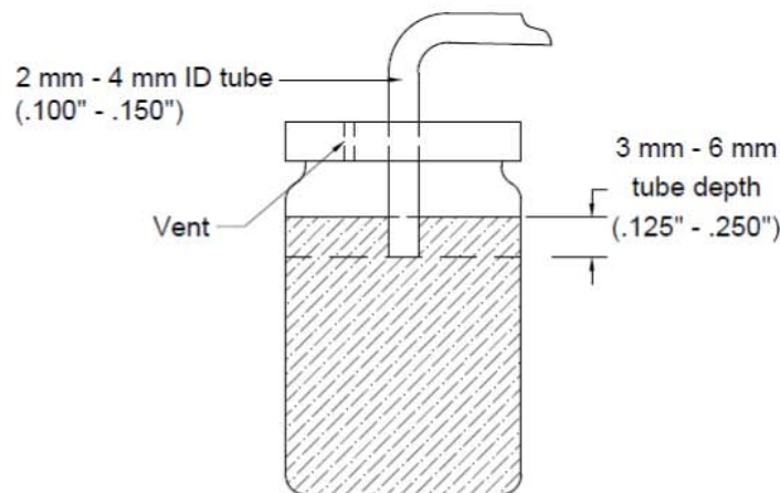
Figure 1—Volumetric Device
